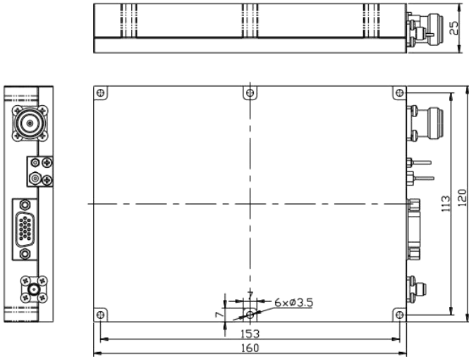
CRF-PA-400M440M-100W-M Outline Drawing
