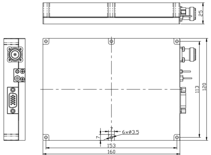
CRF-PA-400M440M-100W-V Outline Drawing
